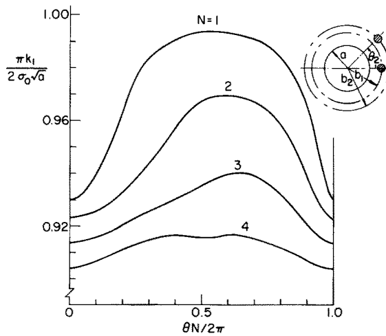
Fig. 8. Angular variation of the stress intensity factor for two sets of reinforcing fibers; b_1 = 1.4a , b_2 = 1.5a , \theta_1 = 0 , \theta_2 = \pi/4 , E_1 = E_2 = 130E , \nu = 0.35 , r_1 = r_2 = 0.2a , N_1 = N_2 = N .
