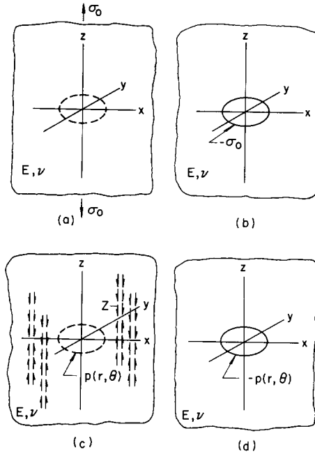
Fig. 2. Superposition for the stresses and displacements in the matrix.
