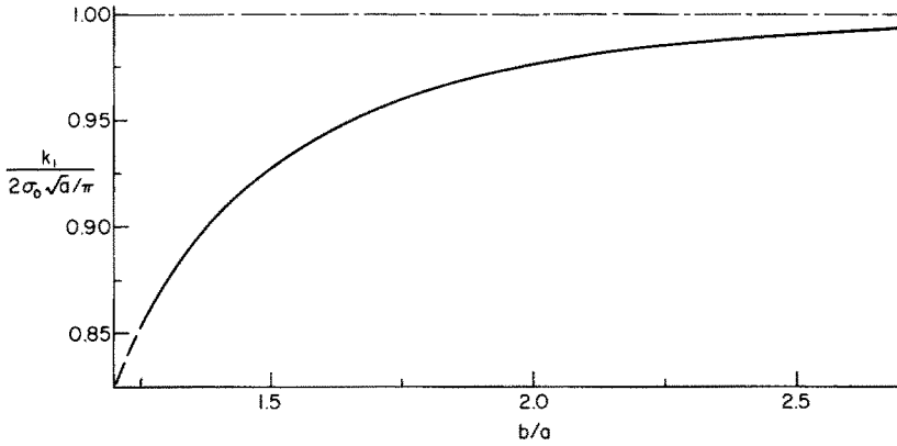
Fig. 6. Effect of the fiber distance b on the stress intensity factor for the axisymmetric case; N = 16 , r_0 = 0.1a , E_f = 130E , \nu = 0.35 .
