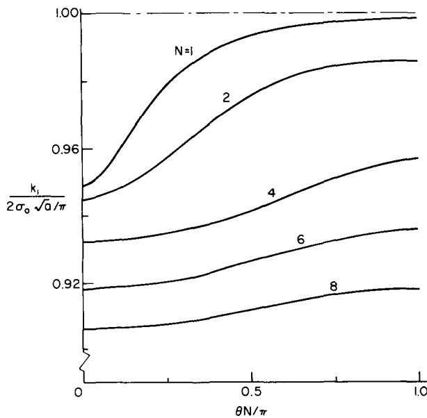
Fig. 5. Effect of the number of fibers N on the stress intensity factor distribution along the crack border; b = 1.375a , r_0 = 0.15a , \nu = 0.35 , E_f = 130E .
