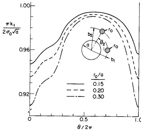
Fig. 7. Angular variation of the stress intensity factor for reinforcement by two fibers; b_1 = 1.4a , b_2 = 1.5a , \theta_1 = 0 , \theta_2 = 0.4\pi , E_1 = E_2 = 130E , \nu = 0.35 , r_1 = r_2 = r_0 , and (—): r_0 = 0.15a , (---): r_0 = 0.20a , (-·-·-): r_0 = 0.30a .
