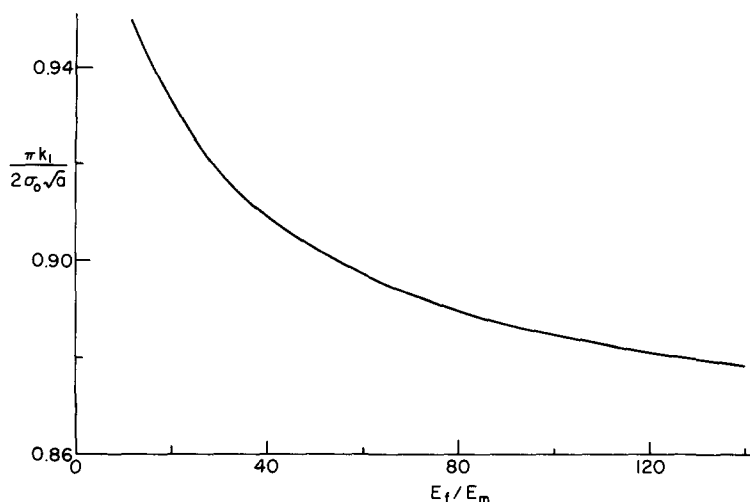
Fig. 12. Effect of modulus ratio E_f/E_m on the stress intensity factor for reinforcement by two sets of fibers obtained from the axisymmetric solutions; E_1 = E_2 = E_f , \nu = 0.35 , N_1 = N_2 = 8 , b_1 = 1.25a , b_2 = 1.5a , r_1 = r_2 = 0.1a .
