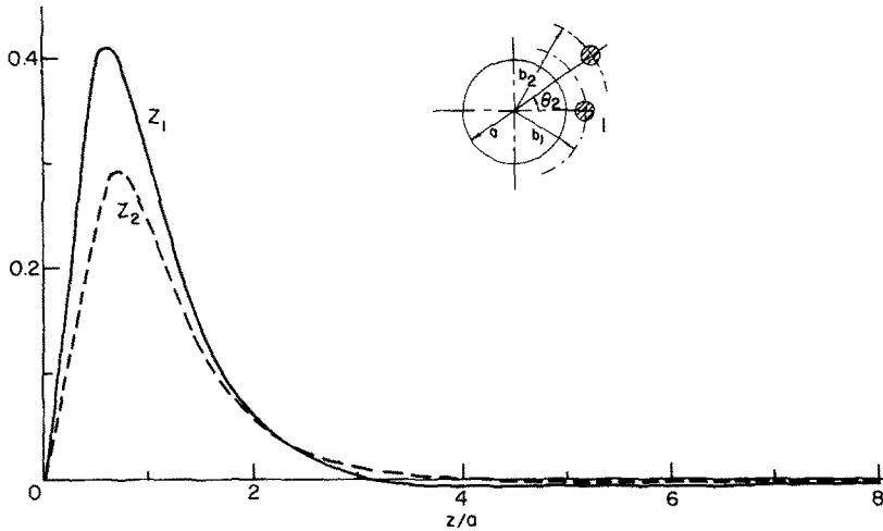
Fig. 9. Distribution of body forces for reinforcement by two fibers; b_1 = 1.5a , b_2 = 1.6a , r_1 = r_2 = 0.4a , \theta_1 = 0 , \theta_2 = 0.2\pi , E_1 = E_2 = 15E .
