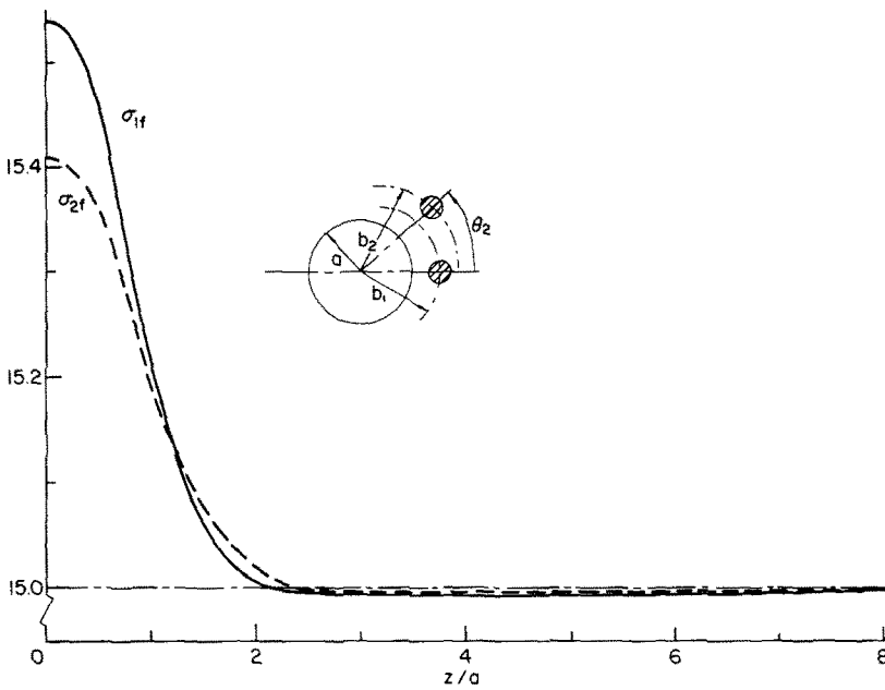
Fig. 10. Distribution of fiber stress \sigma_f for reinforcement by two fibers; b_1 = 1.5a , b_2 = 1.6a , r_1 = r_2 = 0.4a , \theta_1 = 0 , \theta_2 = 0.2\pi , E_1 = E_2 = 15E .
