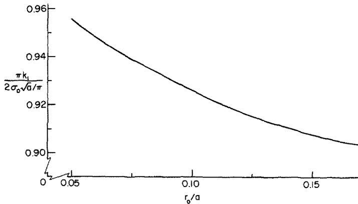
Fig. 11. Effect of fiber radius r_0 = r_1 = r_2 on the stress intensity factor for reinforcement by two sets of fibers obtained from the axisymmetric solution, N_1 = N_2 = 8 , b_1 = 1.4a , b_2 = 1.6a , E_1 = E_2 = 130E , \nu = 0.35 .
