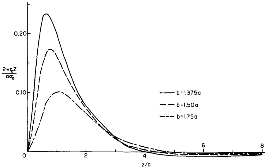
Fig. 4. Distribution of body force Z(z) for E_f = 130E , \nu = 0.35 , r_0 = 0.15a , and (—): b = 1.375a , (---): b = 1.50a , (-·-·-): b = 1.75a .
