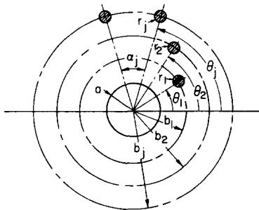
Fig. 3. Geometry of the multiple set of fibers; M is the number of concentric rings containing the fibers; in each ring the fibers are equally spaced with \alpha_j = 2\pi/N_j , N_j being the number of fibers in the j th ring.
