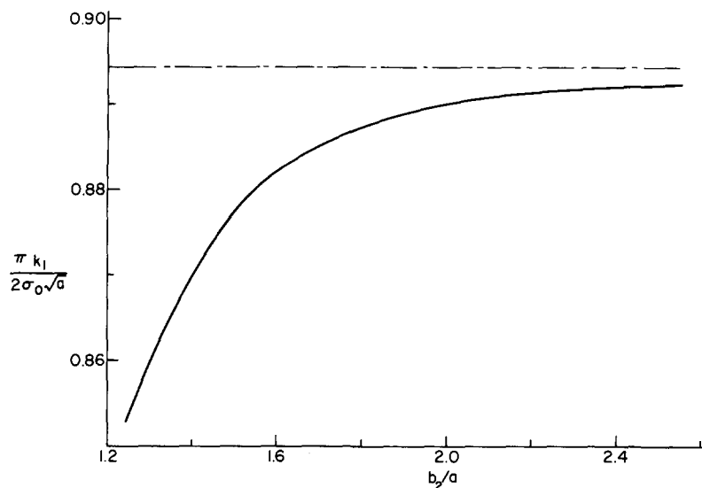
Fig. 13. Effect of fiber distance b_2 on the stress intensity factor for reinforcement by two sets of fibers obtained from the axisymmetric solution; N_1 = N_2 = 8 , E_1 = E_2 = 130E , \nu = 0.35 , b_1 = 1.25a , r_1 = r_2 = 0.1a .
