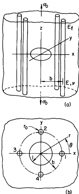
Fig. 1. Geometry for the penny-shaped crack in an elastic matrix reinforced by symmetrically located elastic fibers.
